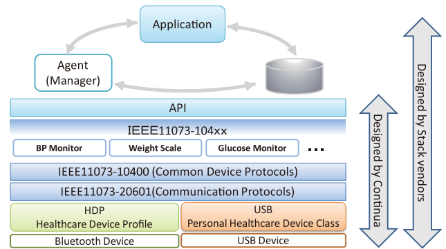
Fig. 3 Protocol stack designed by Continua Health Alliance
