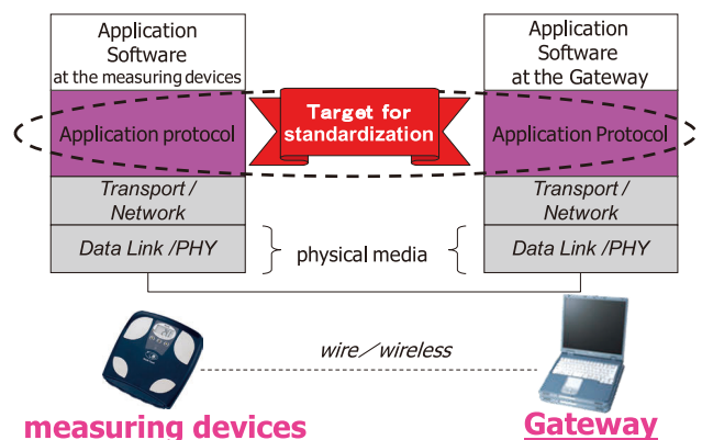
Fig. 2 Protocol stack
