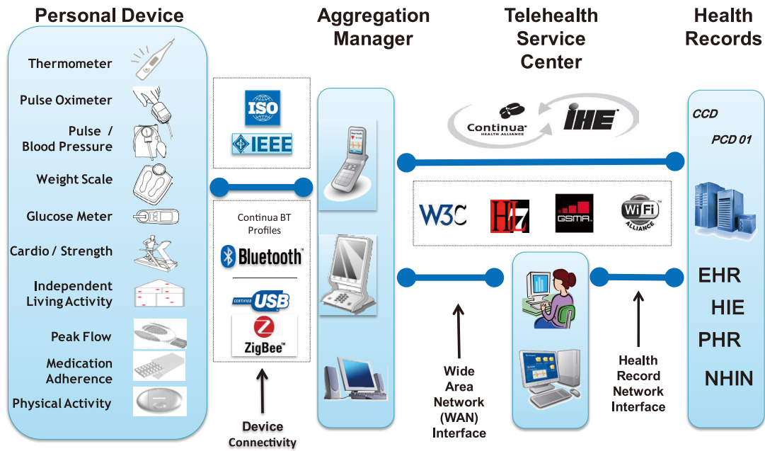
Fig. 4 Interfaces and standards designed by Continua Health Alliance
